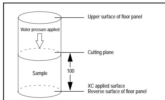
Figure 1: Test sample for water blocking ability
