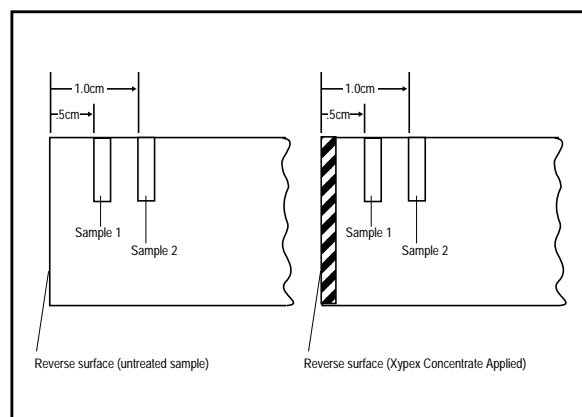
Figure 4: Location for extracting the SEM observation samples.
