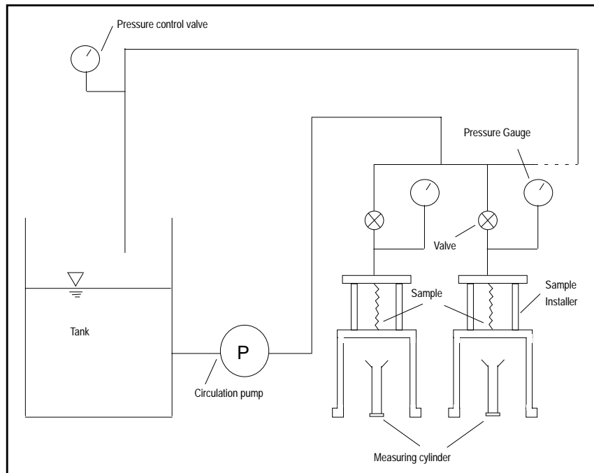
Figure 2: Conceptual structure of the water leak test
